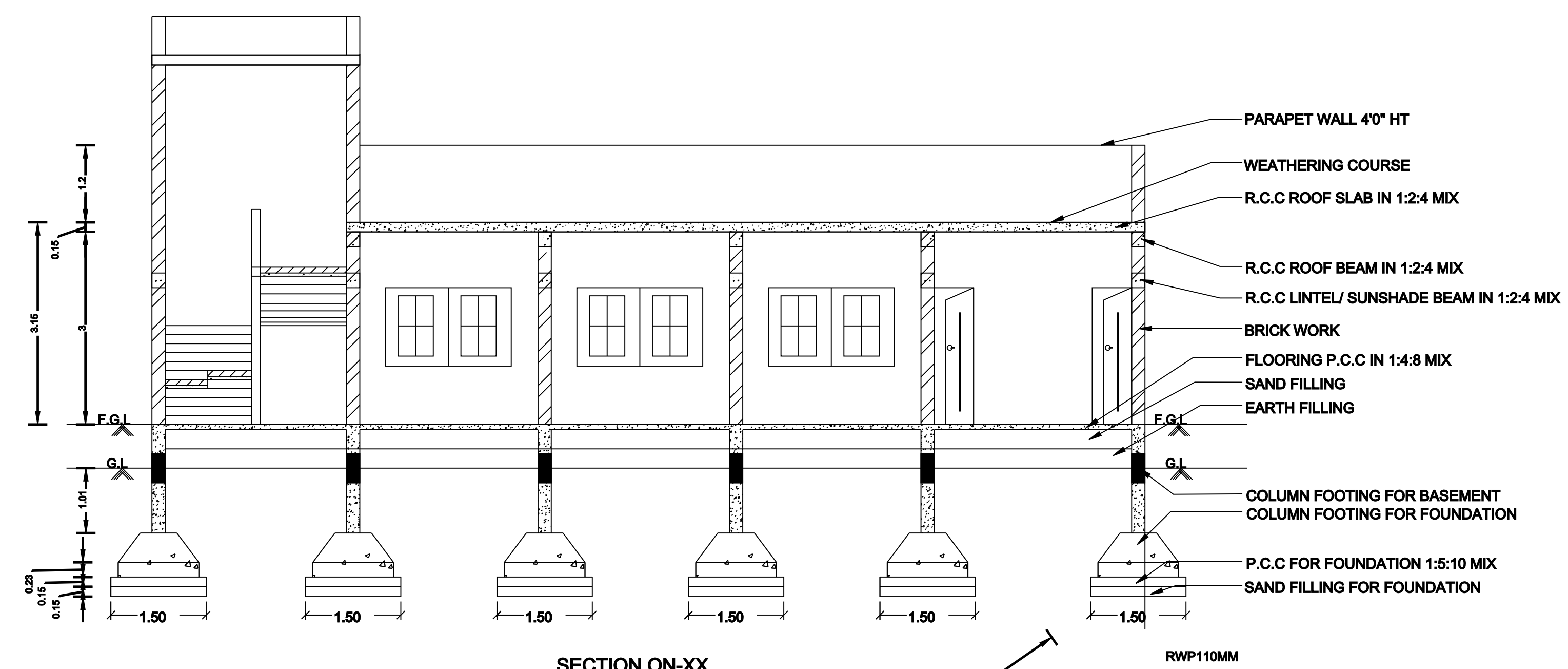
SECTION ON-XX
