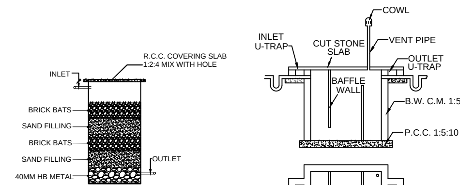
WASTE WATER RECYCLED UNIT
