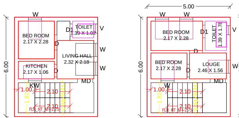
FIRST FLOOR PLAN SECOND FLOOR PLAN
