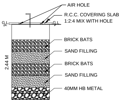
RAINWATER HARVESTING
