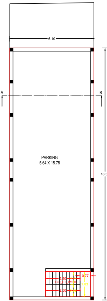
EX.GROUND FLOOR PLAN
