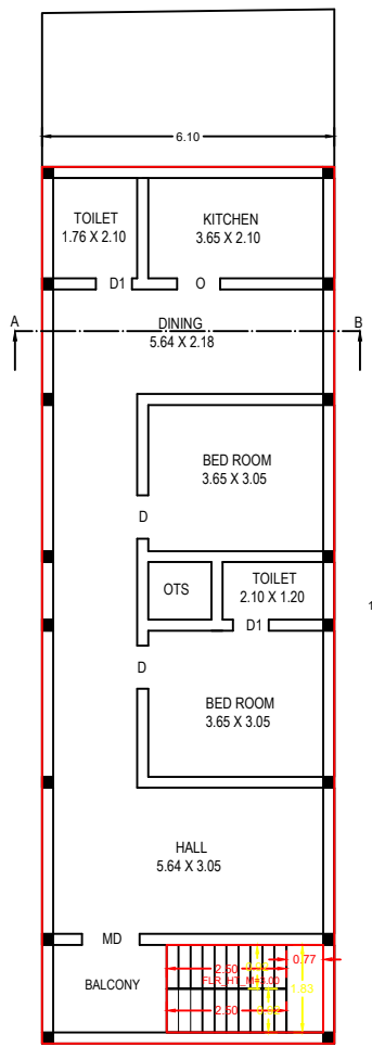
EX.FIRST FLOOR PLAN
