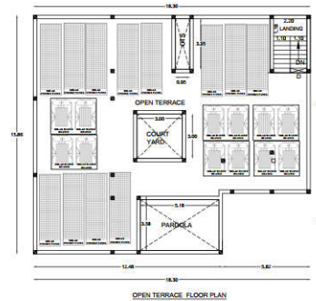
OPEN TERRACE FLOOR PLAN
