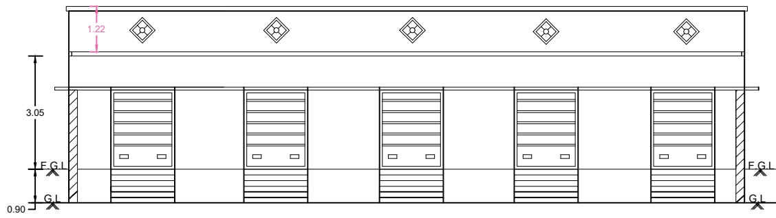
FRONT ELEVATION
