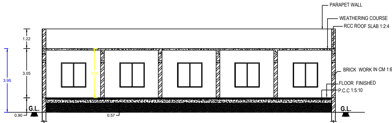
SECTION "A-B"
