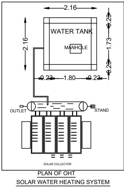
PLAN OF OHT SOLAR WATER HEATING SYSTEM
