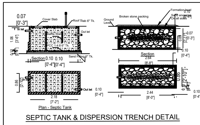
SEPTIC TANK & DISPERSION TRENCH DETAIL
