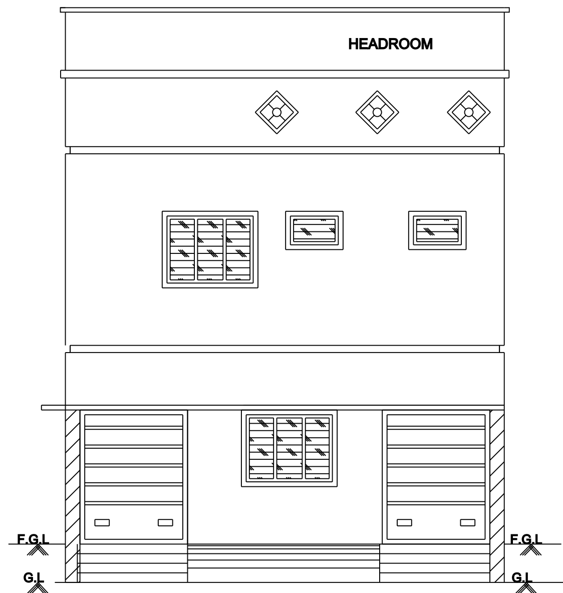
FRONT ELEVATION
