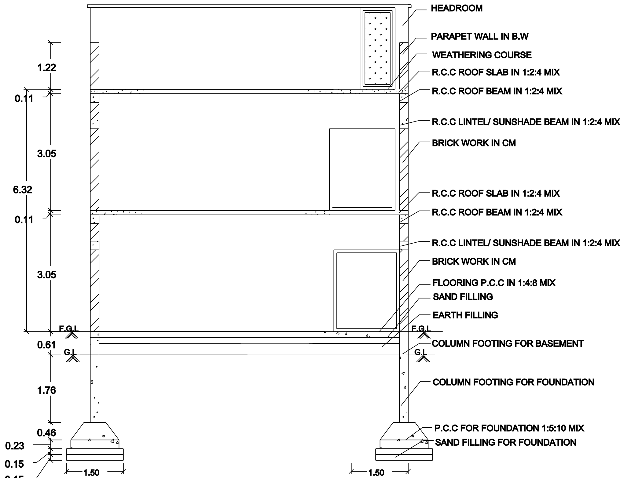
SECTION ON-AA
