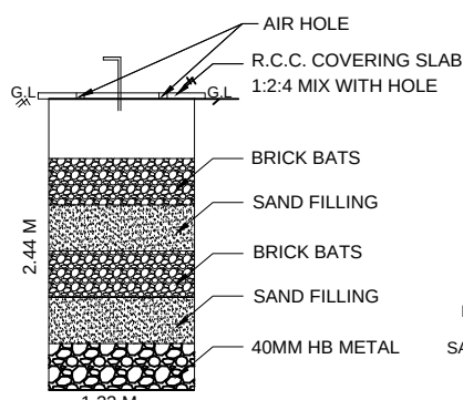
RAINWATER HARVESTING
