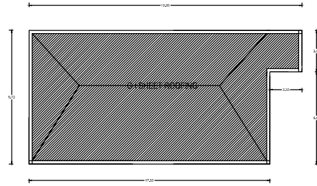
TERRACE PLAN
