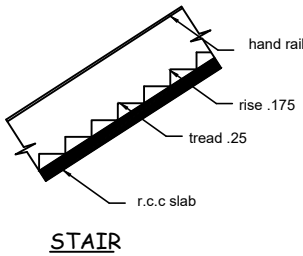
STAIR
