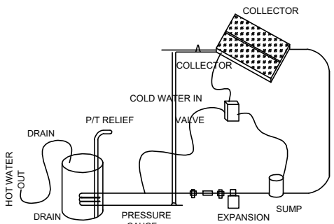
SOLAR WATER HEATER CAPACITY 100lpd
