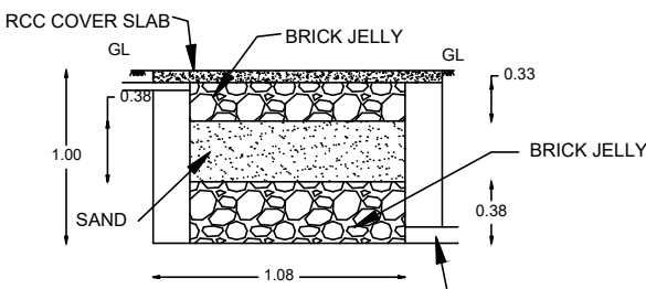
RAIN WATER HARVEST
