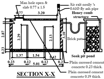
SECTION X-X DETAIL OF SEPTIC TANK (scale -1:200)
