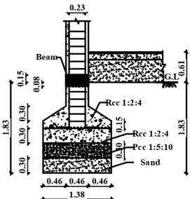
SECTION Z-Z SCALE 1:200
