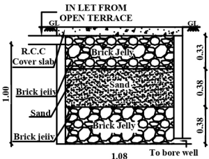
RAIN WATER HARVEST
