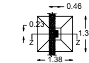
COLUMN FOOTING DETAIL
