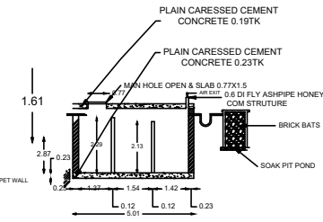
SECTION XX
