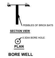
BORE WELL
