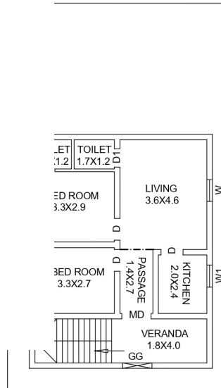
PROPOSED GROUND FLOOR
