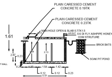
SECTION XX
