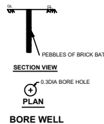
BORE WELL
