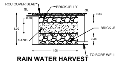
RAIN WATER HARVEST
