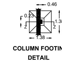
SECTION Z-Z
