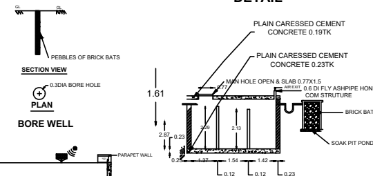
SECTION XX
