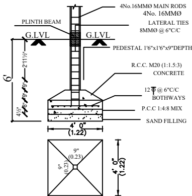
FOUNDATION DETAIL
