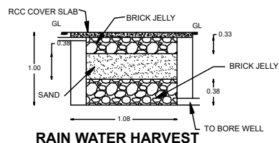
RAIN WATER HARVEST
