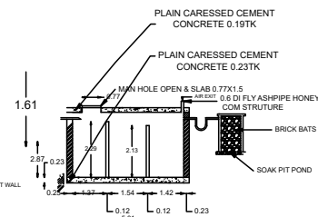
SECTION XX
