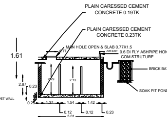
SECTION XX
