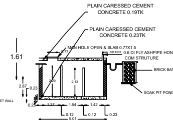
SECTION XX
