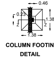
SECTION Z-Z
