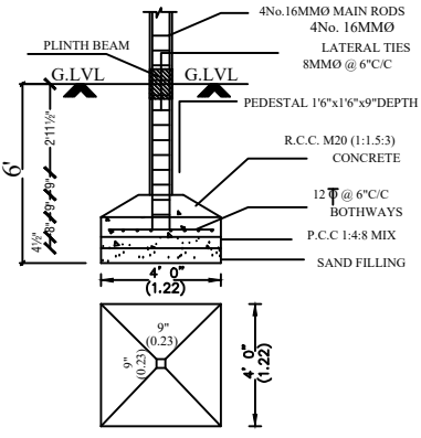
FOUNDATION DETAIL
