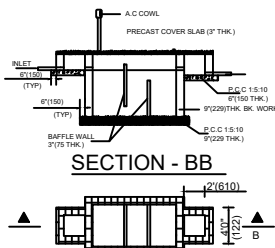
SECTION - BB PLAN OF SEPTIC TANK
