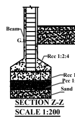
SECTION Z-Z SCALE 1:200
