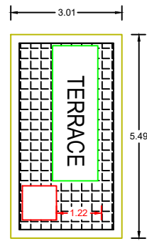
PRO.TERRACE FLOOR PLAN
