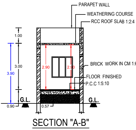
SECTION "A-B"
