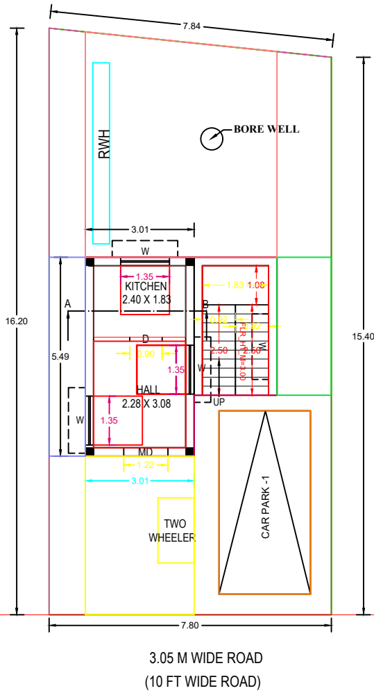
SITE CUM PRO.GROUND FLOOR PLAN
