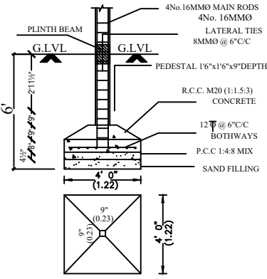
FOUNDATION DETAIL
