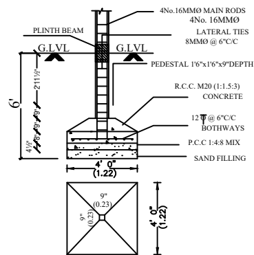
FOUNDATION DETAIL
