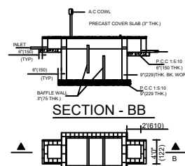
(23) (244) (23) PLAN OF SEPTIC TANK
