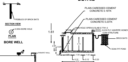
SECTION XX
