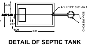
DETAIL OF SEPTIC TANK
