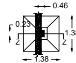
COLUMN FOOTING DETAIL
