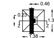
COLUMN FOOTING DETAIL
