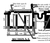
DETAIL OF SEPTIC TANK
