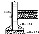
SECTION Z-Z
