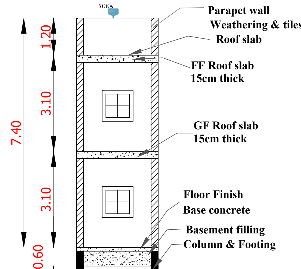
SECTION AA'
