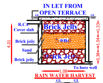
RAIN WATER HARVESTING SCALE 1:100
