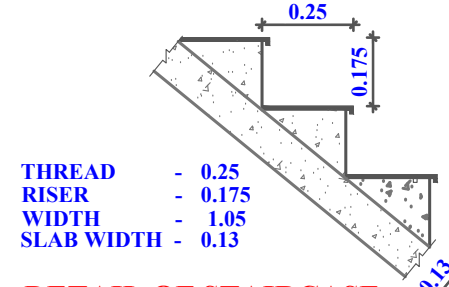
DETAIL OF STAIRCASE SCALE 1:200
