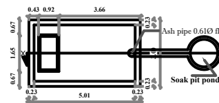
DETAIL OF SEPTIC TANK (scale -1:200)
