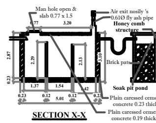
SECTION X-X
