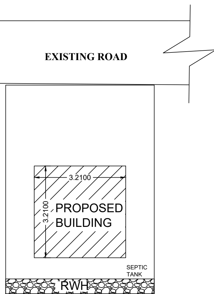
SITE PLAN
