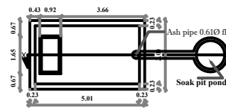
DETAIL OF SEPTIC TANK (scale -1:200)
