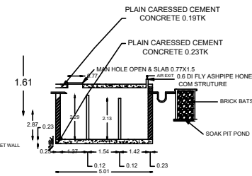
SECTION XX
