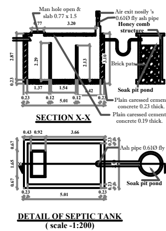
RAIN WATER HARVEST
