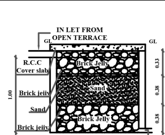
RAIN WATER HARVEST
