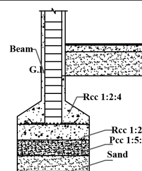
SECTION Z-Z SCALE 1:200
