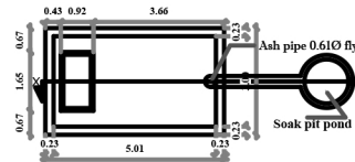
DETAIL OF SEPTIC TANK (scale -1:200)
