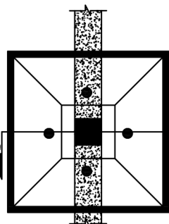
COLUMN FOOTING DETAIL
