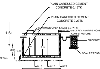
SECTION XX
