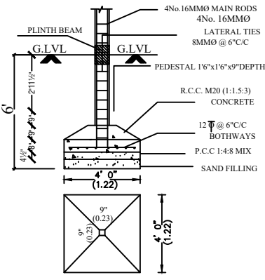
FOUNDATION DETAIL
