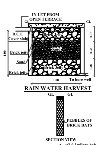
RAIN WATER HARVESTING SCALE 1:100
