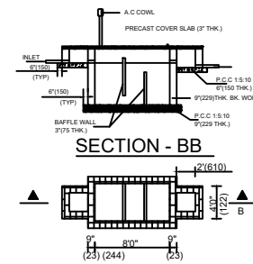
(20) (244) (20) PLAN OF SEPTIC TANK
