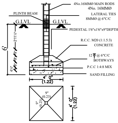
FOUNDATION DETAIL
