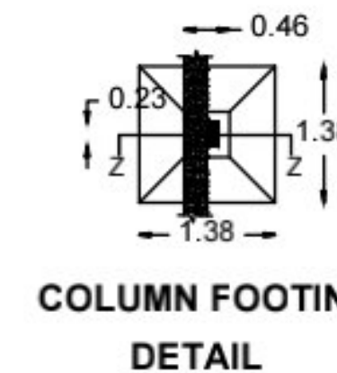
SECTION Z-Z
