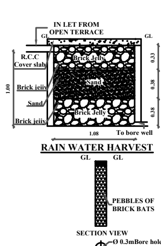
RAIN WATER HARVESTING SCALE 1:100
