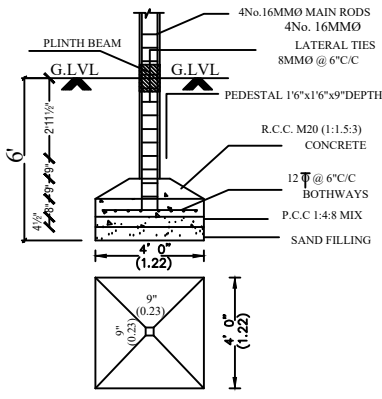
FOUNDATION DETAIL
