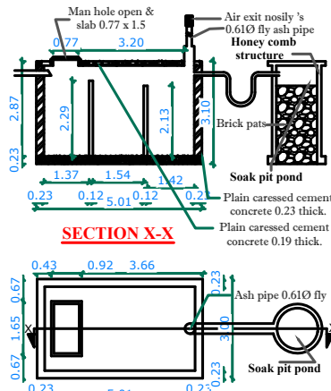
DETAIL OF SEPTIC TANK (scale -1:200)
