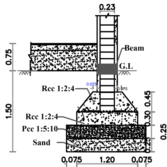
SECTION Z-Z' SCALE 1:200
