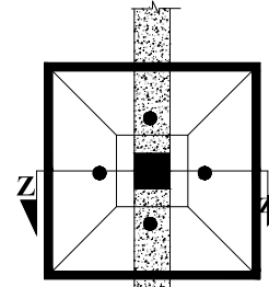
COLUMN FOOTING DETAIL
