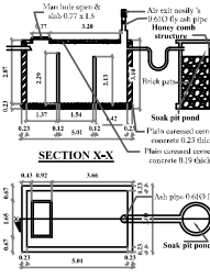
DETAIL OF SEPTIC TANK (scale-1:200)
