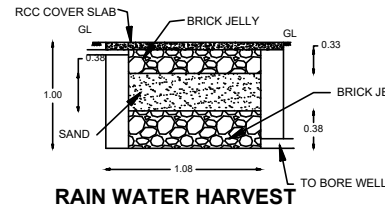
RAIN WATER HARVEST
