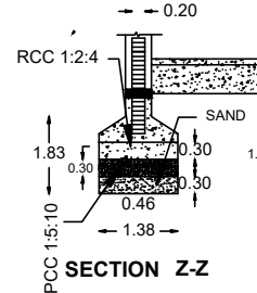
DETAIL OF STAIRCASE
